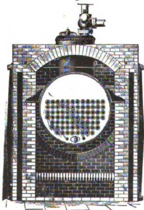
FIG. 20.—SECTION OF TUBULAR BOILER AND SETTING.
